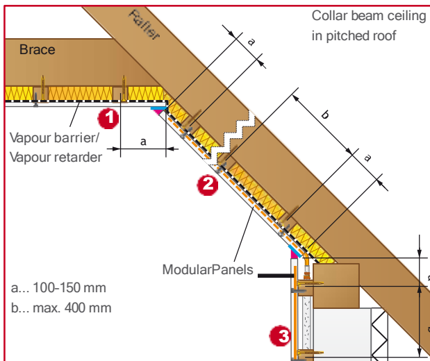
Cross-section - horizontal battens
