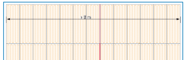
▲ Movement joint at e.g. 13× V020-100 ( 13 \times 0.625 \text{ m} = 8.13 \text{ m} )
