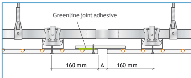
▲ Movement joint with panel strips, A = 10\text{-}20 \text{ mm} (movement dimension)
