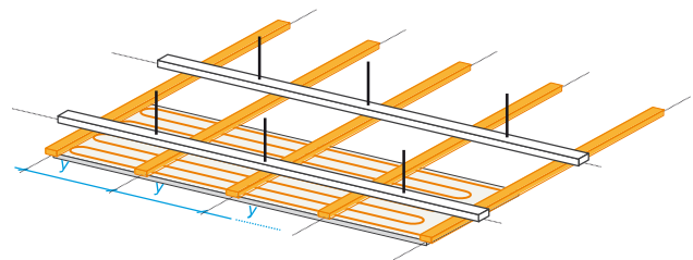
▲ Cross joists transverse to the ModularPanels
