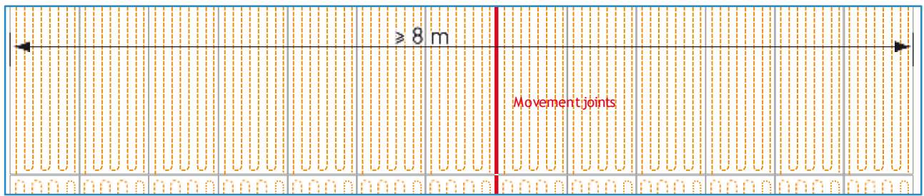
▲ Movement joint at e.g. 13x V020-100 (13x0.625 m = 8.13 m)
