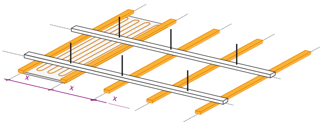
▲ Cross joists longitudinal to the ModularPanels
