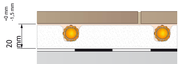
▲ System height and tolerances
